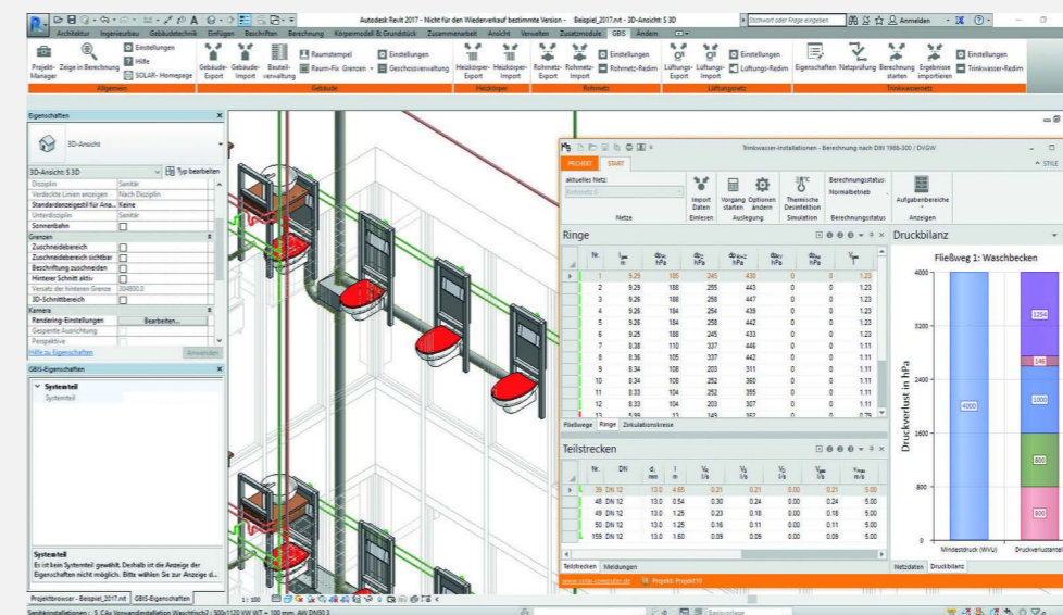
Fig. 31 GBIS ribbons, GBIS properties, and SOLAR-COMPUTER calculation program dialogs are fully integrated into the Revit interface. Examples: Heating Load EN 12831-1, Heating Pipe Network, Drinking Water Installation DIN 1988-300.
