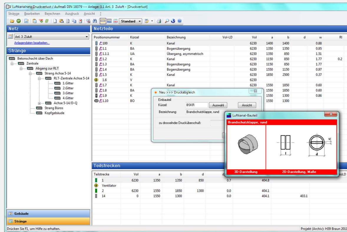
Fig. 16 Inspecting and editing the runs, subsections, and network components of an air duct system for calculating pressure loss and balancing. Fully integrated with duct measurement mode.
